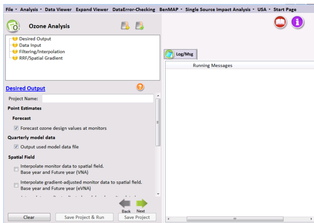
Figure 8-2. Choose Desired Output for Ozone Analysis
